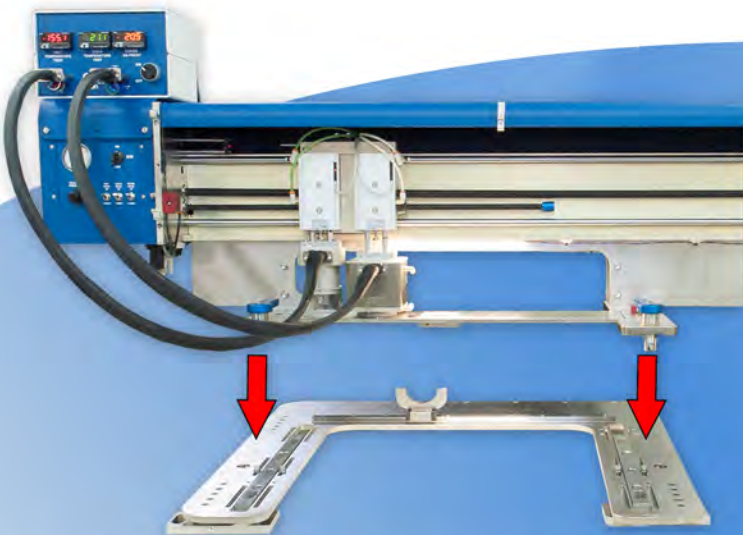
Thermal Test Heads and Removable Test Site Dock
